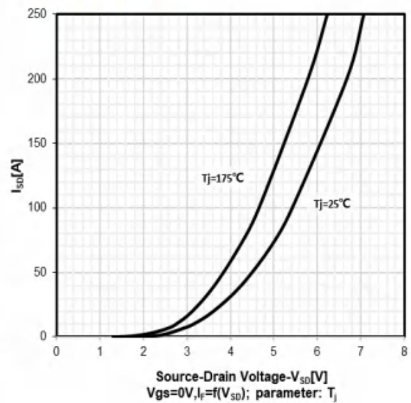
Diode forward voltage characteristics T_j=25\text{ }^\circ\text{C}/175\text{ }^\circ\text{C}
