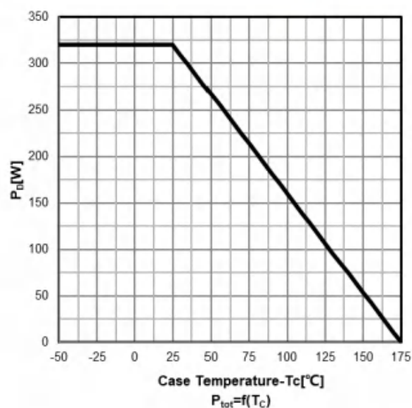
Power dissipation
