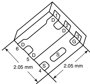
DFN2X2
