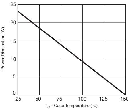
Power Derating
