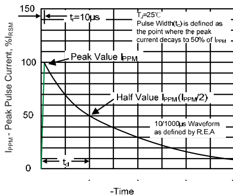
Figure 3. Pulse Waveform
