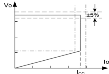
Fig.1. Typical CC/CV Curve
