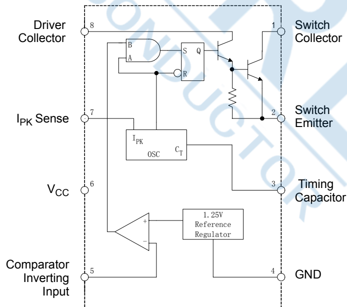
Figure 3. Functional Block Diagram of MC34063
