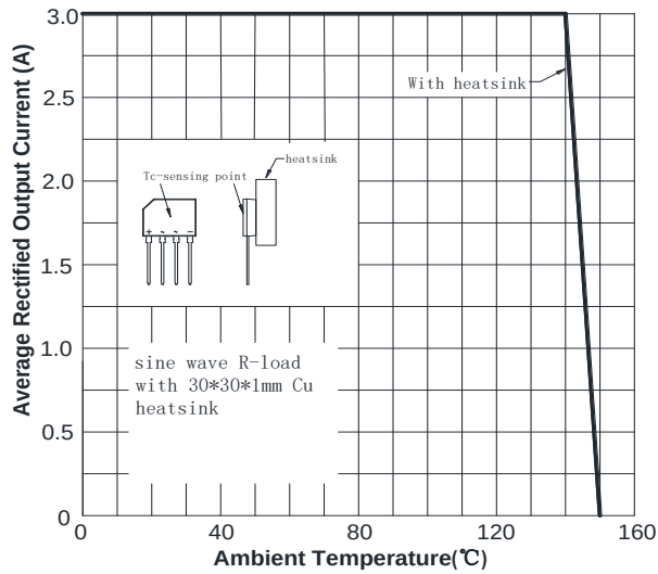
FIG1:Io-Tc Curve
