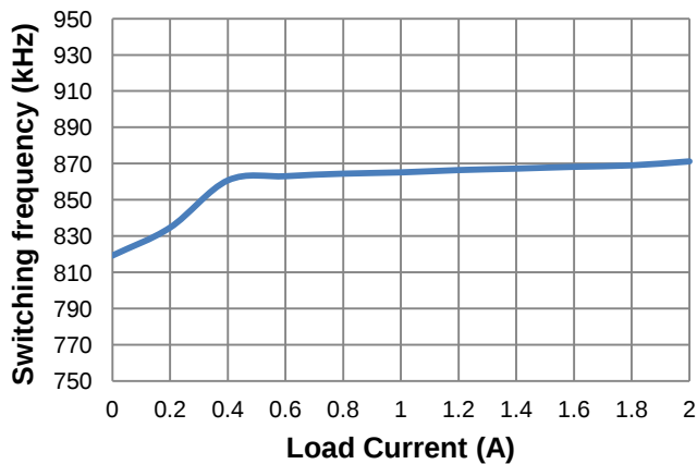
Figure 8. Switch Frequency vs. Load Current
