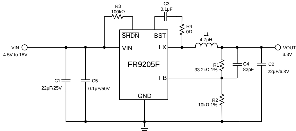
Figure 2. FR9205F Application Circuit
