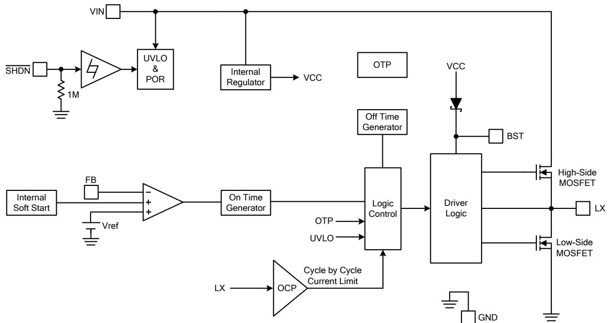
Figure 3. Block Diagram of FR9205F
