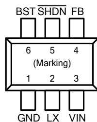
Figure 1. Pin Assignments of FR9205F
