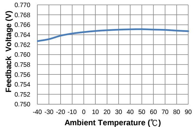
Figure 9. Feedback voltage vs. Temperature
