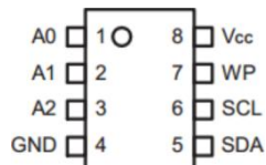
8 - lead SOP
