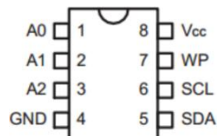
8 - lead DIP
