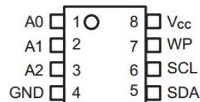
8 - lead MSOP
