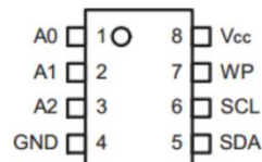
8 - lead TSSOP
