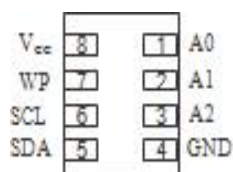
8 - lead DFN
