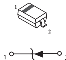
SOD-123
