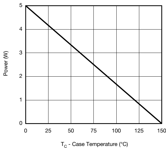
Power, Junction-to-Foot
