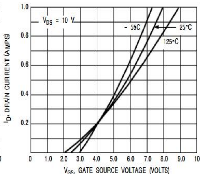
Figure 2. Transfer Characteristics
