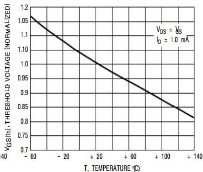
Figure 4. Temperature versus Gate Threshold Voltage
