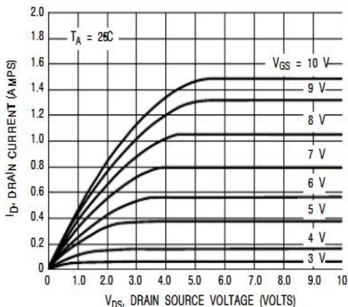
Figure 1. Ohmic Region
