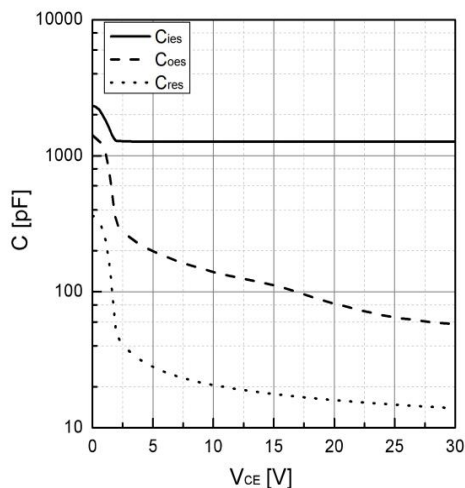
Fig 13. Typical capacitance as a function of V_C ( f=1\text{Mhz} , V_{GE}=0\text{V} )
