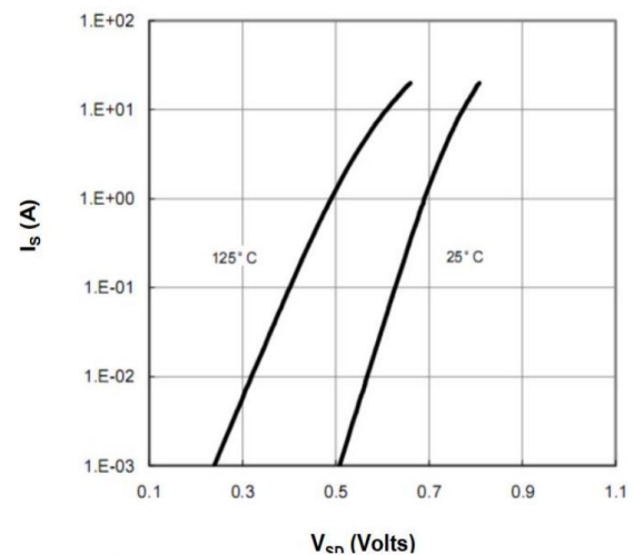
Figure 6: Body-Diode Characteristics
