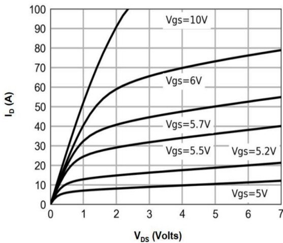
Figure 1: On-Region Characteristics
