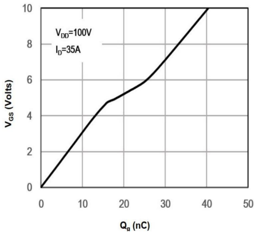
Figure 7: Gate-Charge Characteristics
