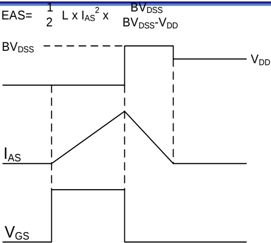
Fig.8 EAS Waveform
