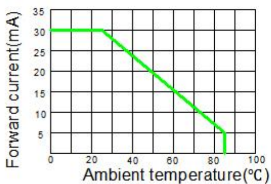
Current and ambient temperature
