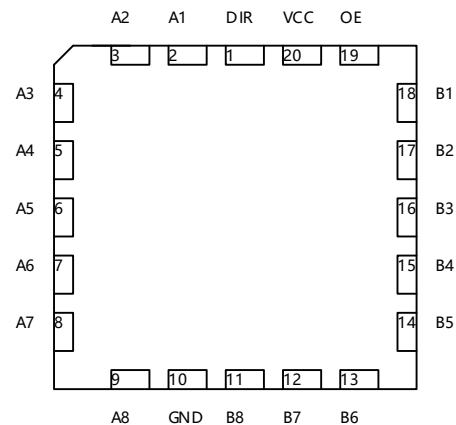
QFN20(4X4)
