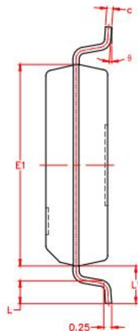
RIGHT-VIEW:
