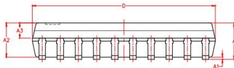
FRONT-VIEW:
