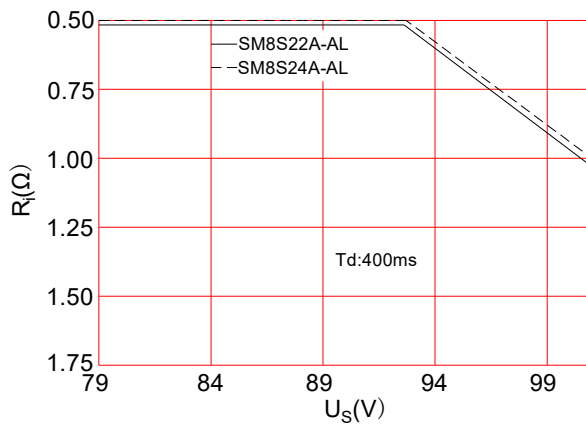
FIG.9: Typical SOA chart ISO16750-2 5A 12V test system
