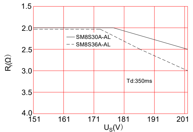
FIG.10: Typical SOA chart ISO16750-2 5A 24V test system
