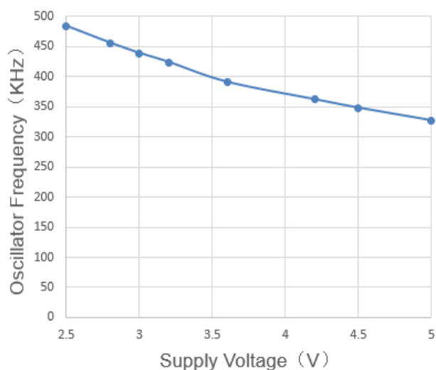
Oscillator Frequency vs. Supply Voltage (I LOAD =0mA)
