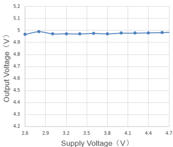
Output Voltage vs. Supply Voltage (I LOAD =0mA)
