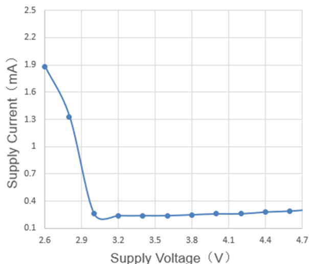
Supply Current vs. Supply Voltage (I LOAD =0mA)
