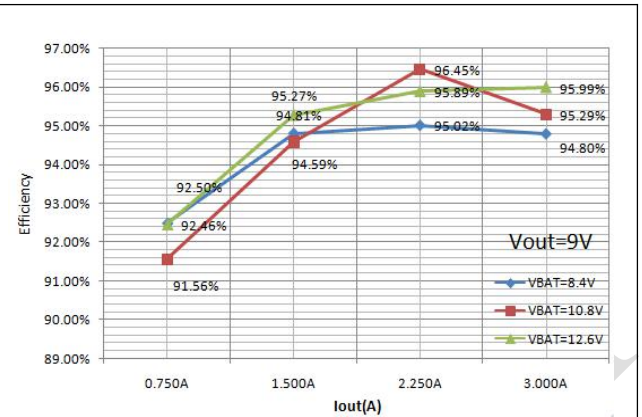
Fig. 4 Efficiency
