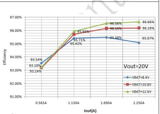
Fig. 4 Efficiency
