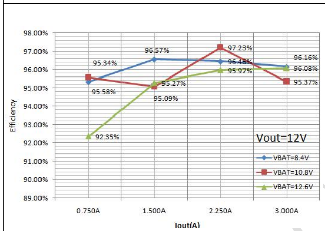
Fig. 3 Efficiency
