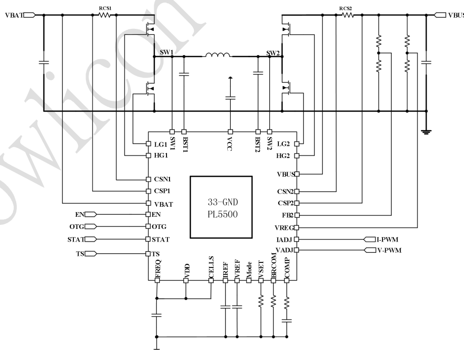
Fig. 1 Application Schematic
