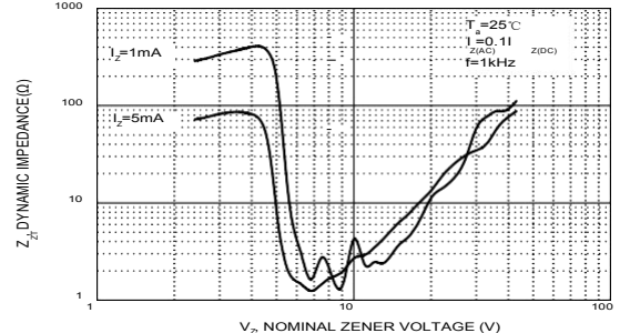
Effect of Zener Voltage on Zener Impedance
