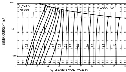
Zener Characteristics ( V_Z Up to 10 V)
