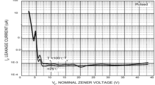
Typical Leakage Current
