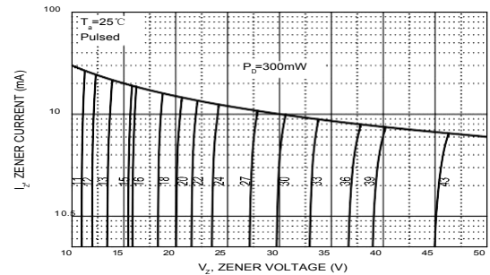
Zener Characteristics (11 V to 43 V)
