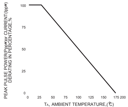
FIG. 2-PULSE DERATING CURVE
