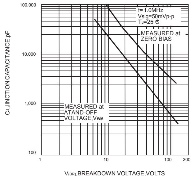
FIG. 4-TYPICAL JUNCTION CAPACITANCE
