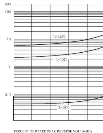
FIG.4-TYPICAL REVERSE CHARACTERISTICS
