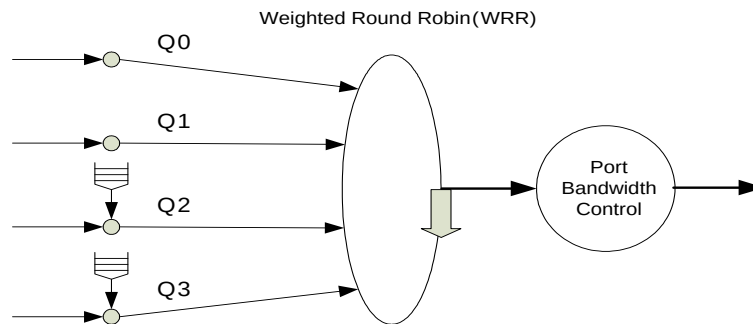
Figure 14. Packet-Scheduling Diagram
