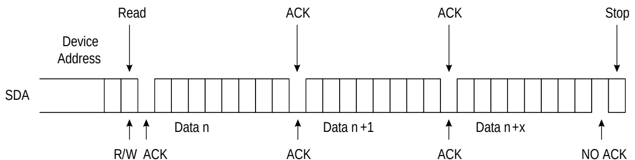
Figure 9. Sequential Read
