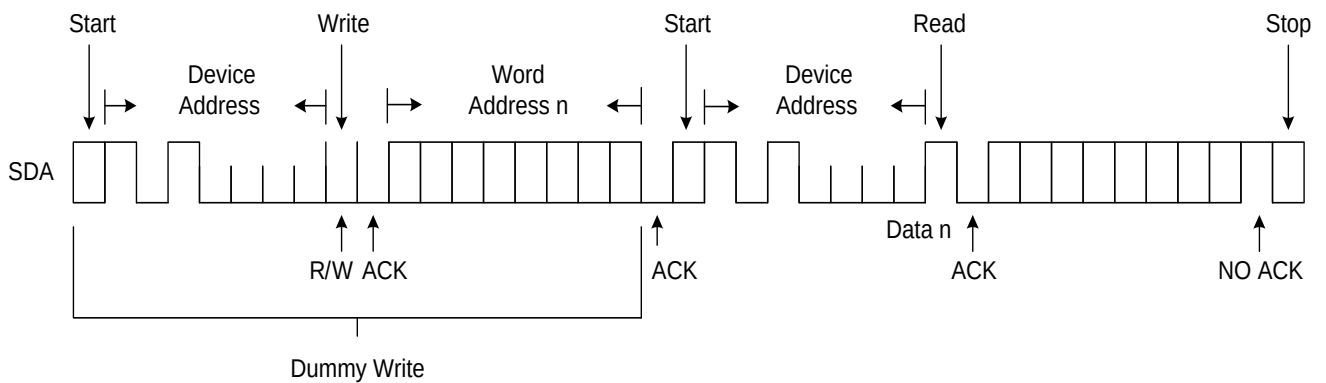
Figure 8. Random Read
