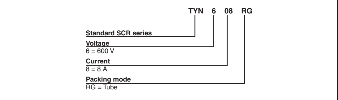
Figure 17. TYNx08 series
