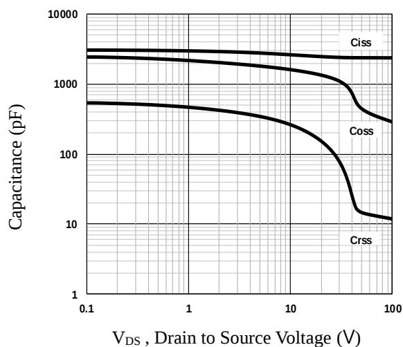
Fig.7 Capacitance Characteristics
