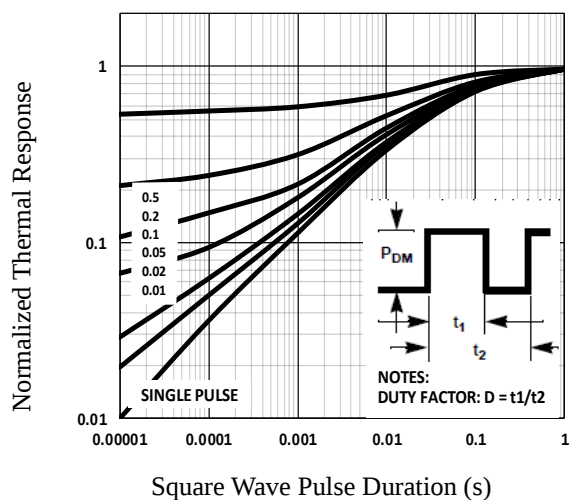
Fig.11 Normalized Transient
