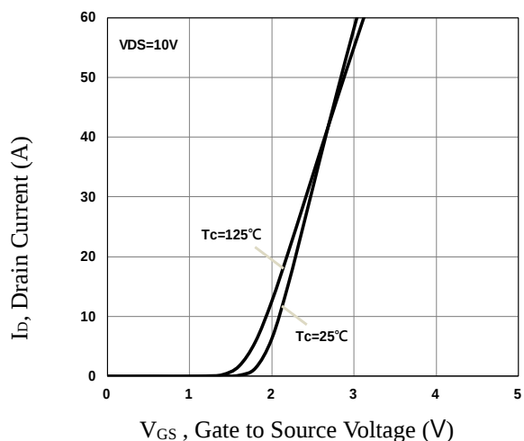
Fig.9 Transfer Characteristics
