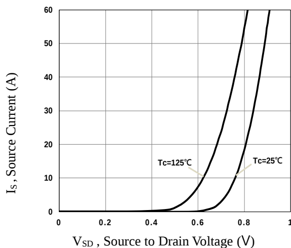
Fig.10 Source Current vs. V_{SD}
