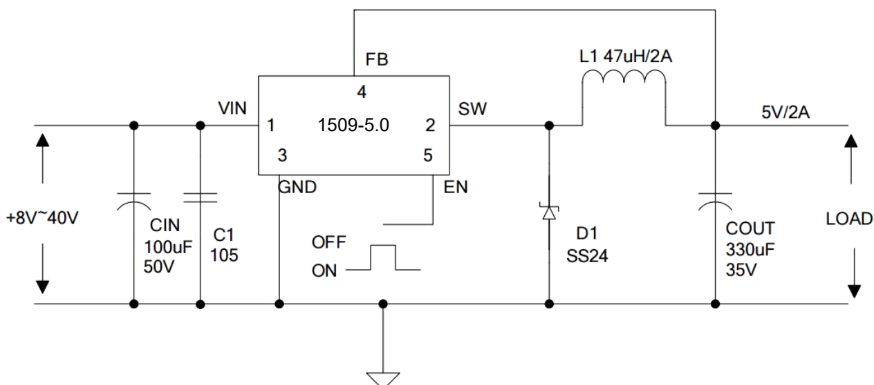
Figure2. HXL1509-5.0 Typical Application Circuit (VIN=8V~40V, VOUT=5V/2A)
