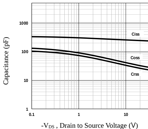
Fig.19 Capacitance Characteristics
