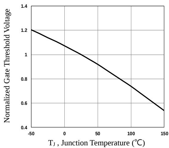
Fig.16 Normalized V_{th} vs. T_J
