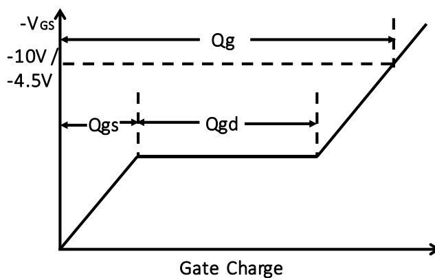
Fig.24 Gate Charge Waveform
