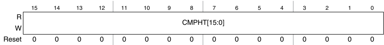
Figure 13-13. ATD Compare Higher Than Register (ATDCMPHT)
