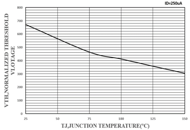
FIG 4.GATE THRESHOLD VOLTAGE
