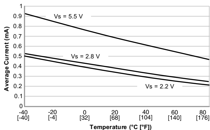
SL353HT Typical Average Current vs Temperature
