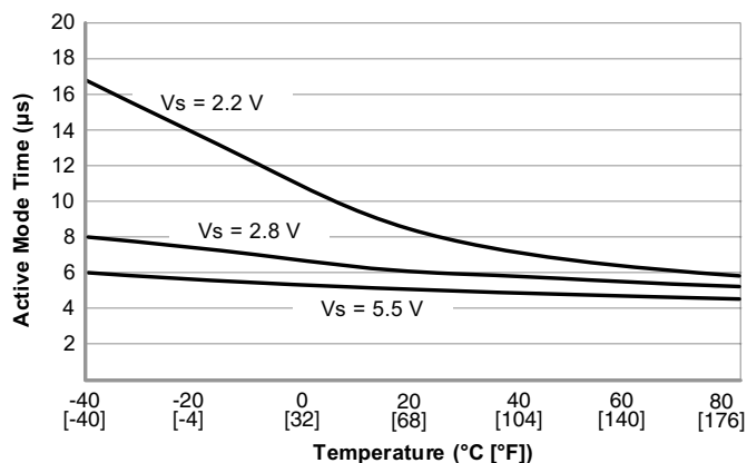
SL353HT and SL353LT Typical Active Mode Time vs Temperature
