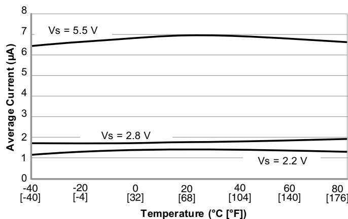
SL353LT Typical Average Current vs Temperature
