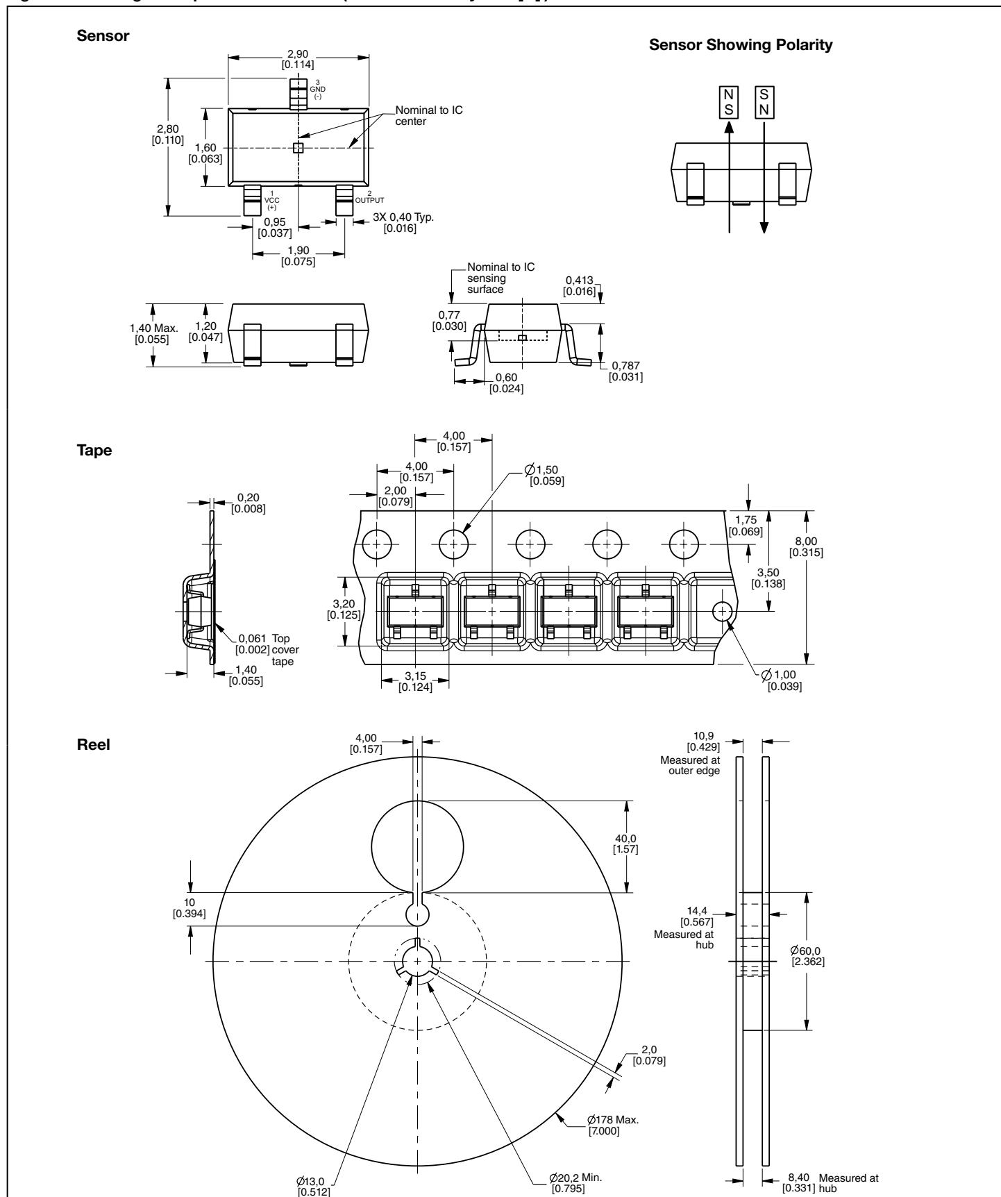
Figure 3. Mounting and Tape/Reel Dimensions (For reference only. mm/[in].)
