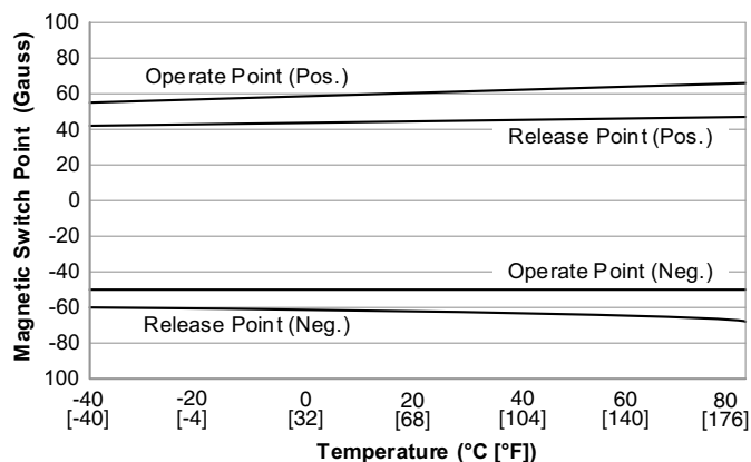
SL353HT and SL353LT Typical Magnetic Performance vs Temperature
