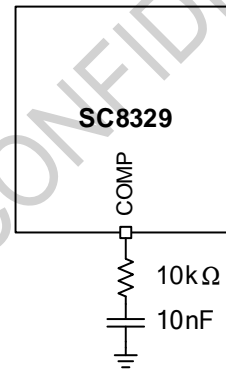
Figure 4. Feedback loop setting
