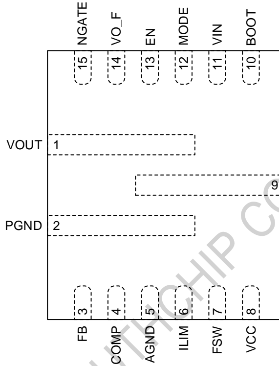
QFN-15 Package Hotrod Top view
