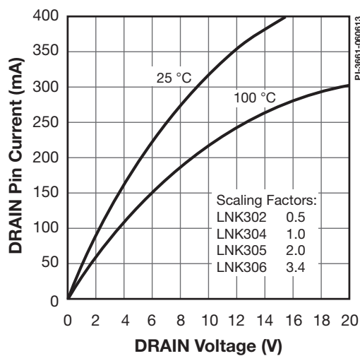
Figure 15. Output Characteristics.
