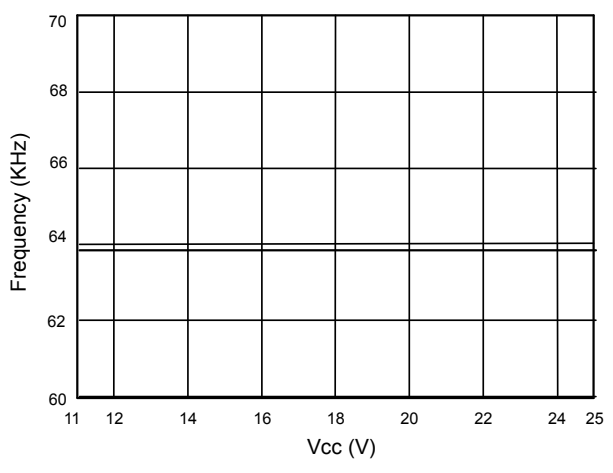
Fig. 7 Frequency vs. Vcc
