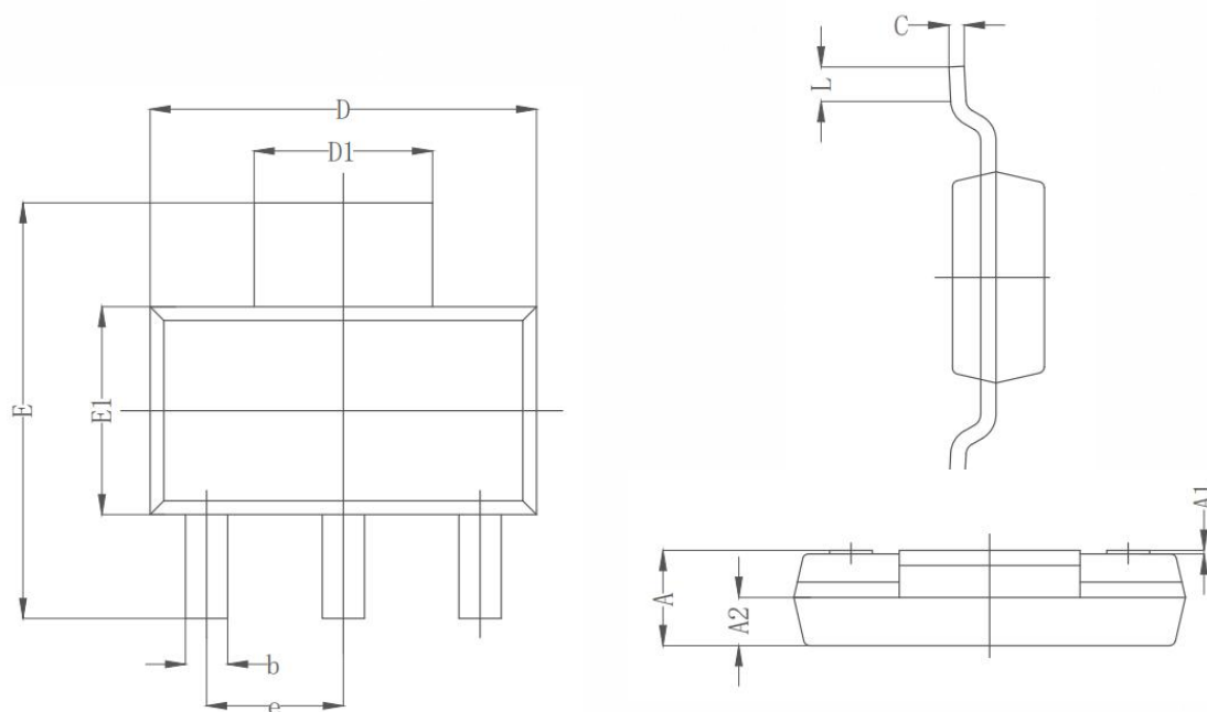
COMMON DIMENSION(MM)
