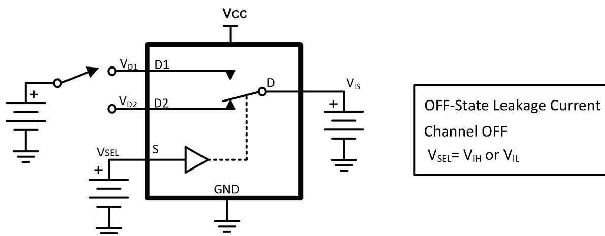
Figure 2. OFF-State Leakage Current
