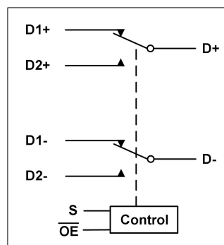
Simplified Schematic
