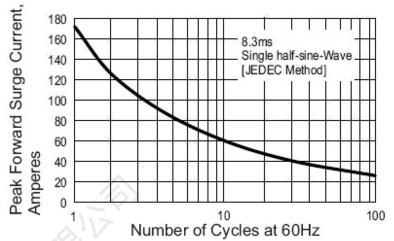
Fig. 2 Maximum Non-repetitive Peak Forward Surge Current
