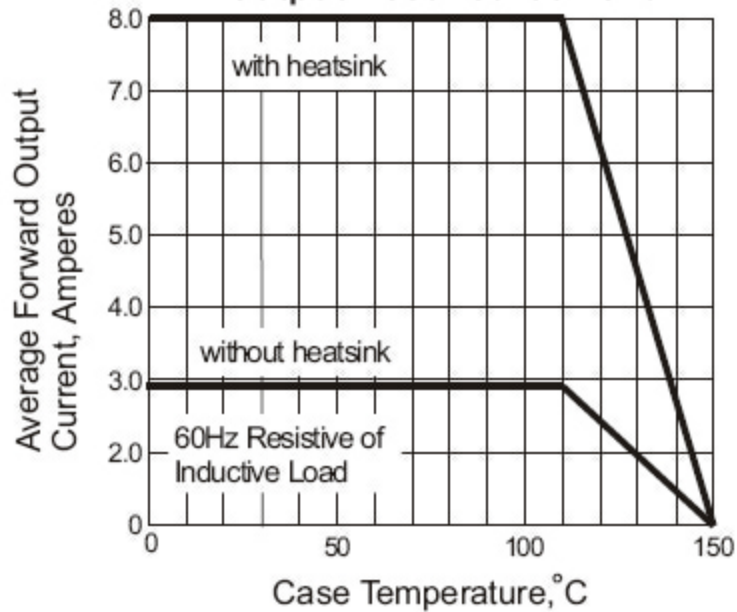
Fig. 1 Derating Curve for Output Rectified Current
