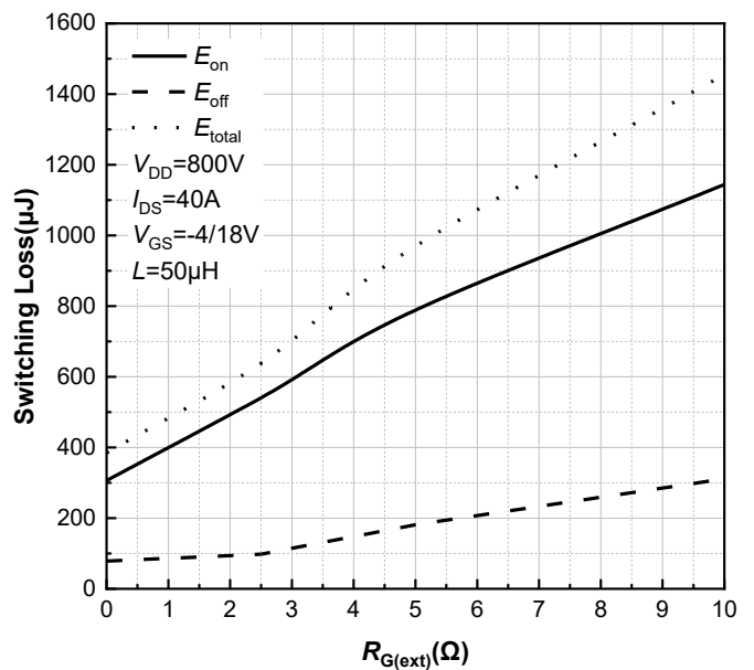
Figure 24. Clamped Inductive Switching Energy vs. R_{G(ext)} T_j=175^\circ\text{C}
