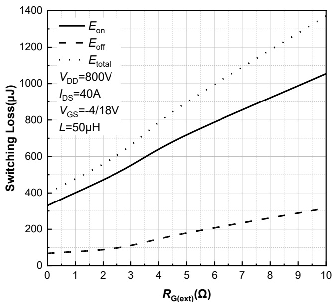
Figure 23. Clamped Inductive Switching Energy vs. R_{G(ext)} T_j=25^\circ\text{C}
