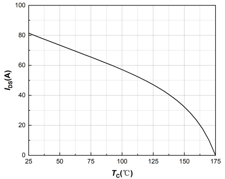
Figure 18. Continuous Drain Current Derating vs. Case Temperature
