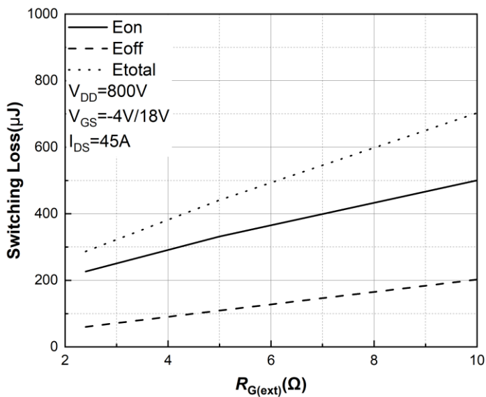
Figure 23. Clamped Inductive Switching Energy vs. R_{G(\text{ext})} T_j = 25^\circ\text{C}
