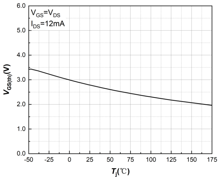
Figure 11. Threshold Voltage vs. Temperature
