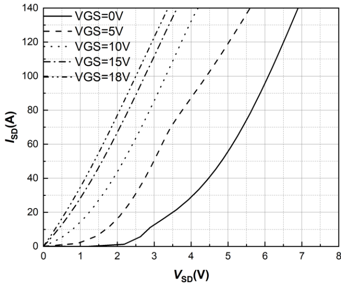
Figure 13. 3rd Quadrant Characteristic T_j = -55^\circ\text{C}
