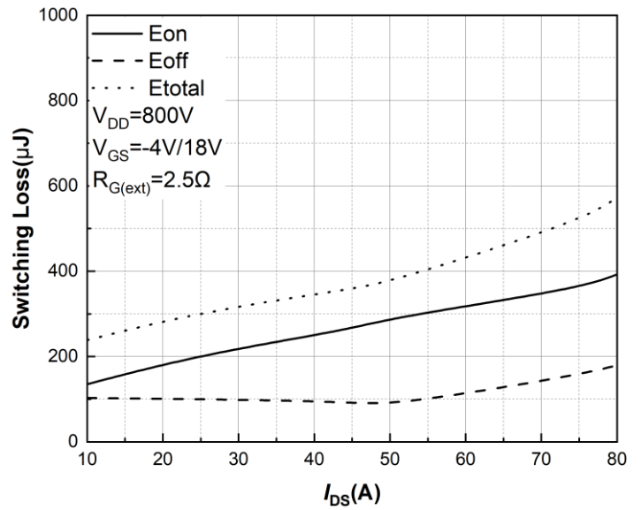
Figure 22. Clamped Inductive Switching Energy vs. Drain Current T_j = 175^\circ\text{C}
