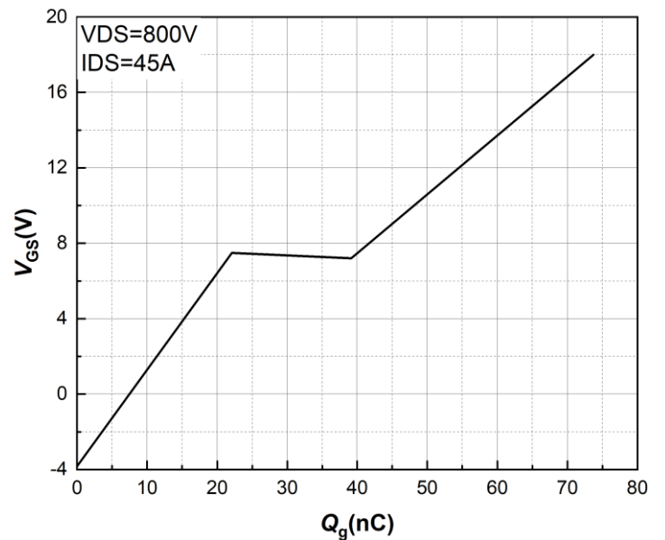
Figure 12. Gate Charge Characteristics
