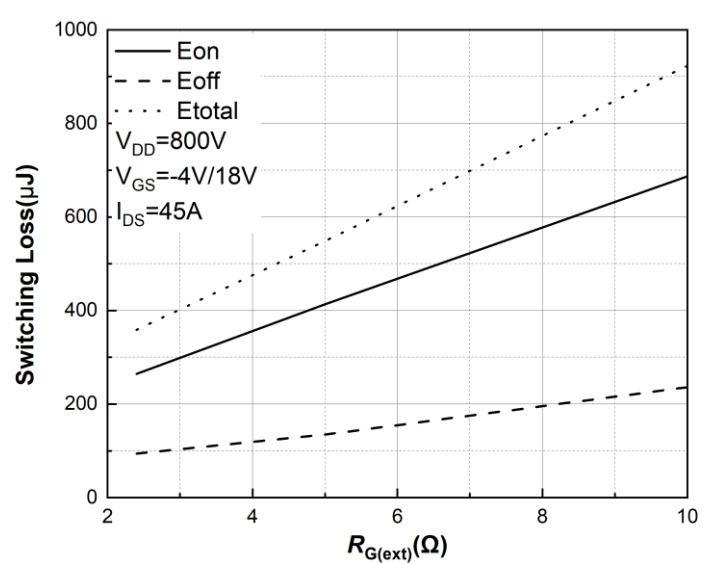
Figure 24. Clamped Inductive Switching Energy vs. R_{G(\text{ext})} T_j = 175^\circ\text{C}
