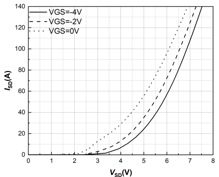
Figure 8. Body Diode Characteristic T_J = -55^\circ\text{C}
