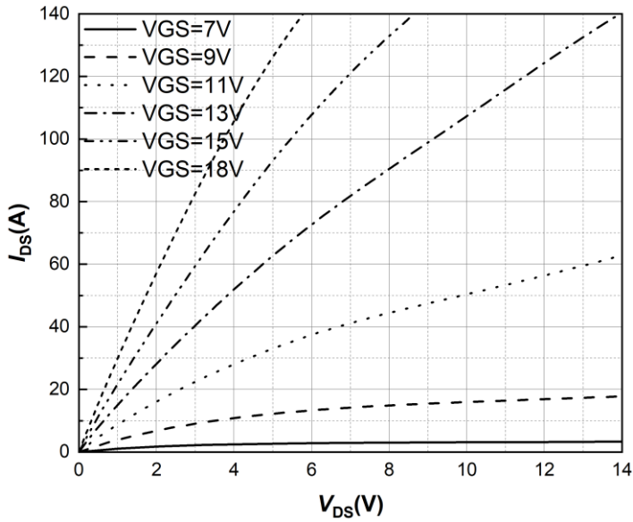
Figure 1. Output Characteristics T_j = -55^{\circ}\text{C}
