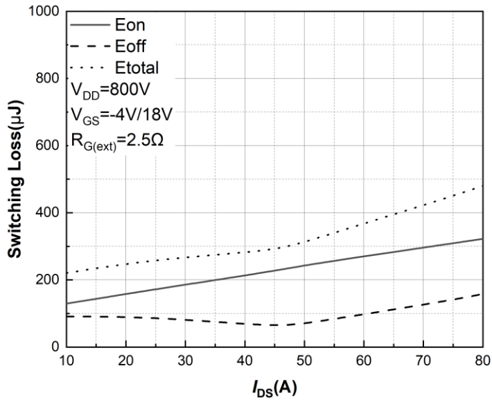
Figure 21. Clamped Inductive Switching Energy vs. Drain Current T_j = 25^\circ\text{C}
