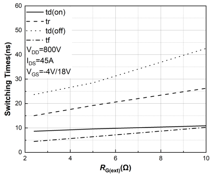
Figure 26. Switching Times vs. R_{G(ext)} T_J = 175^\circ\text{C}
