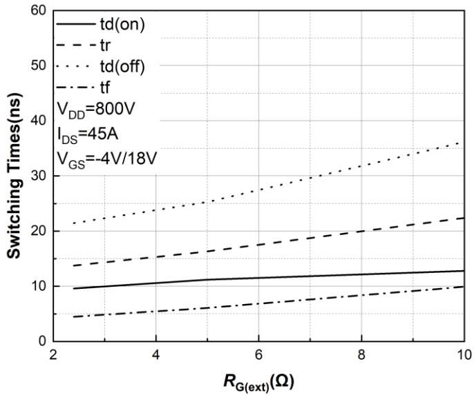
Figure 25. Switching Times vs. R_{G(ext)} T_J = 25^\circ\text{C}
