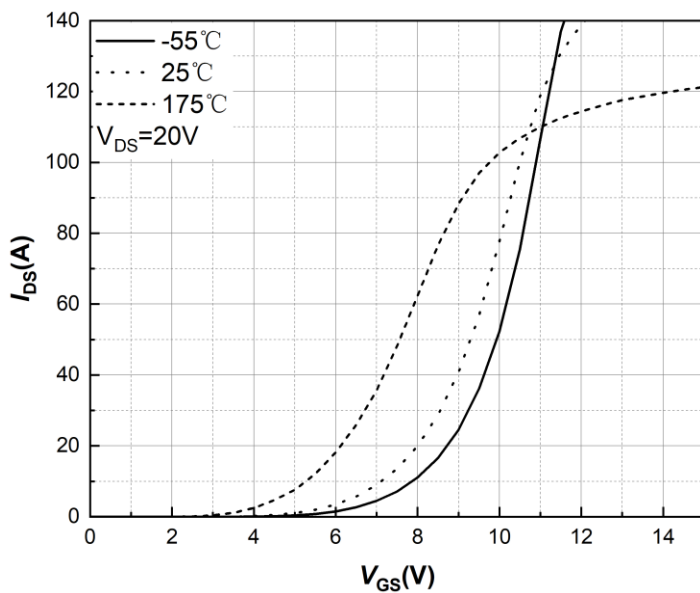
Figure 7. Transfer Characteristic for Various Junction Temperatures
